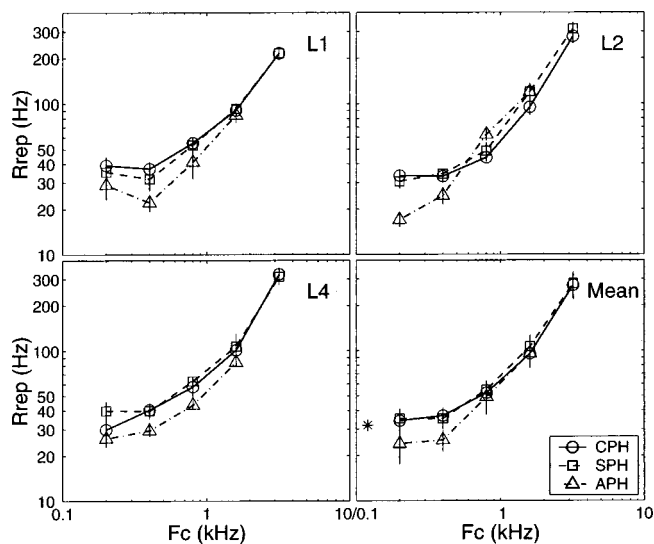
FIG. 2. Results for experiments II and III. The lowest repetition rate, R_{\text{rep}} , of the base note for which the melody task could be performed is plotted as a function of filter cutoff, F_c . The parameter is phase condition (CPH for experiment II, SPH and APH for experiment III). The star symbol on the bottom right panel is the mean result for broadband clicks (experiment I).
