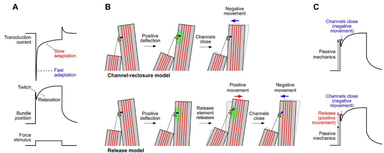
Figure 4. Fast Adaptation
