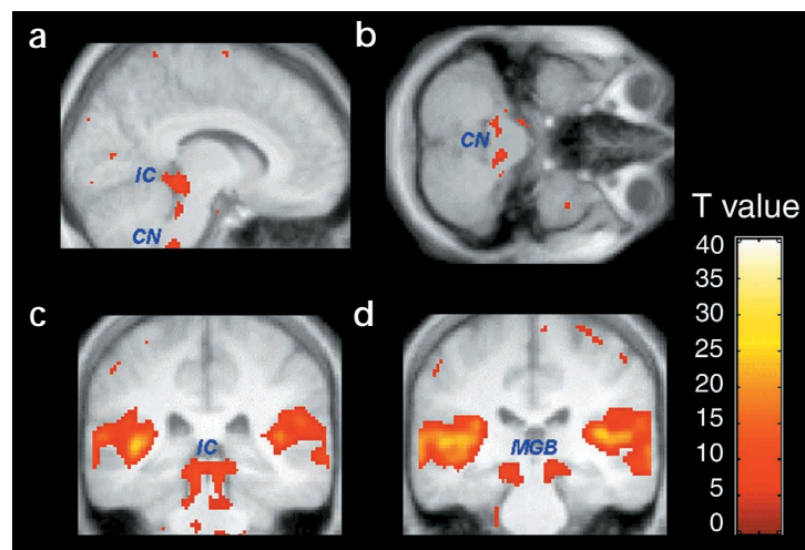
Fig. 2. Activation of structures in the ascending auditory pathway with sound stimuli using cardiac triggering and sparse imaging (contrast between all sound stimuli and silence shown in relation to average structural MRI). Sagittal section at x = 10 mm showing activation in the right cochlear nucleus and inferior colliculus (a), axial section at z = -46 mm showing bilateral activation of cochlear nuclei (b), coronal section at y = -34 mm showing activation of inferior colliculi and superior temporal cortex (c), coronal section at y = -28 mm showing activation of medial geniculate bodies (d). Threshold for contrast p < 0.001 (uncorrected). Color scale gives Student's t statistic for the comparison between the BOLD values in the sound conditions and rest.
