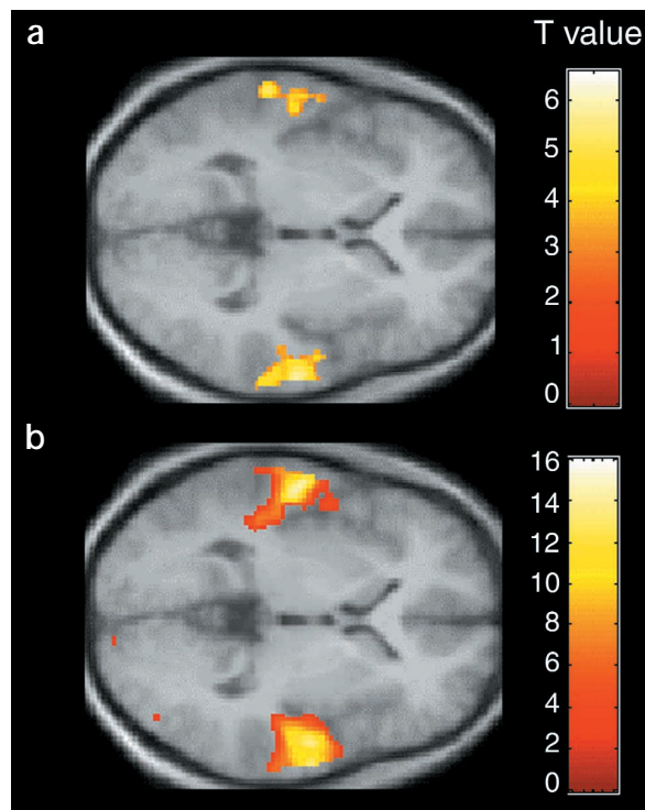
Fig 3. Activation during the processing of the pitch changes between sounds and the temporal structure within sounds. (a) Contrast between the 'lively' pitch sequences and a fixed pitch sequence. Axial section at z = 0 mm. Significant activation is shown in secondary auditory cortex in lateral Heschl's gyrus and cortex posterior to Heschl's gyrus in the plana temporale. No significant activation differences were demonstrated in the brainstem or thalamus. (b) For comparison, the contrast between regular interval sound and noise at the same axial level. This shows activation extending along the whole of Heschl's gyrus including primary auditory cortex in the medial part. Threshold for contrasts, p < 0.001 (uncorrected).
