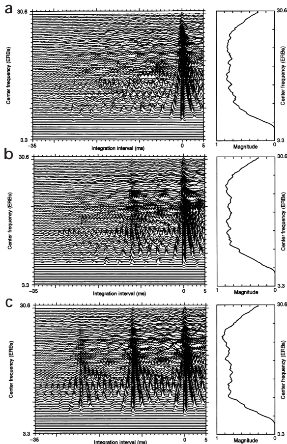
Fig. 1. Experimental protocol. Examples of the internal representations of regular-interval noise from a time-domain model (left) and a spectral model (right). Top, response to a noise stimulus (no temporal regularity and no pitch); middle, response to an intermediate degree of temporal regularity and a weak pitch; bottom, response when there is a high degree of temporal regularity and a strong pitch. Right panel in each row shows sum of the neural activity over time in each channel (a spectral model); no clear pattern of energy peaks emerges with the increase in the temporal regularity of the sound. Left panel in each row shows the 'auditory image' from a time domain model in which the temporal regularity is measured by a form of autocorrelation. A vertical structure centered at the delay (12 ms) emerges as the temporal regularity increases. ERB, equivalent rectangular bandwidth (absolute frequency scale based on the ear's frequency analysis).
